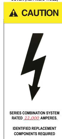
Figure 14 When series ratings are used in a panelboard or switchboard, 110.22 requires the series rating value, such as 22,000 amperes, be field marked on the assembly.
