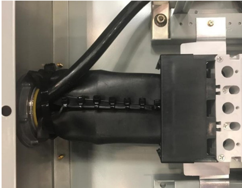
Lineside barrier provides protection from incidental contact.
