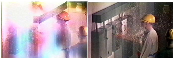
3-phase arcing fault current interrupted in six cycles.
