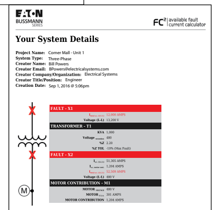
Example of FC 2 Available Fault Current Calculator documentation (right) and electronic formatting of label to affix on equipment (above).
